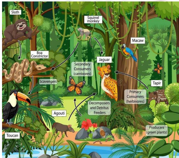
FOREST ECOSYSTEM
