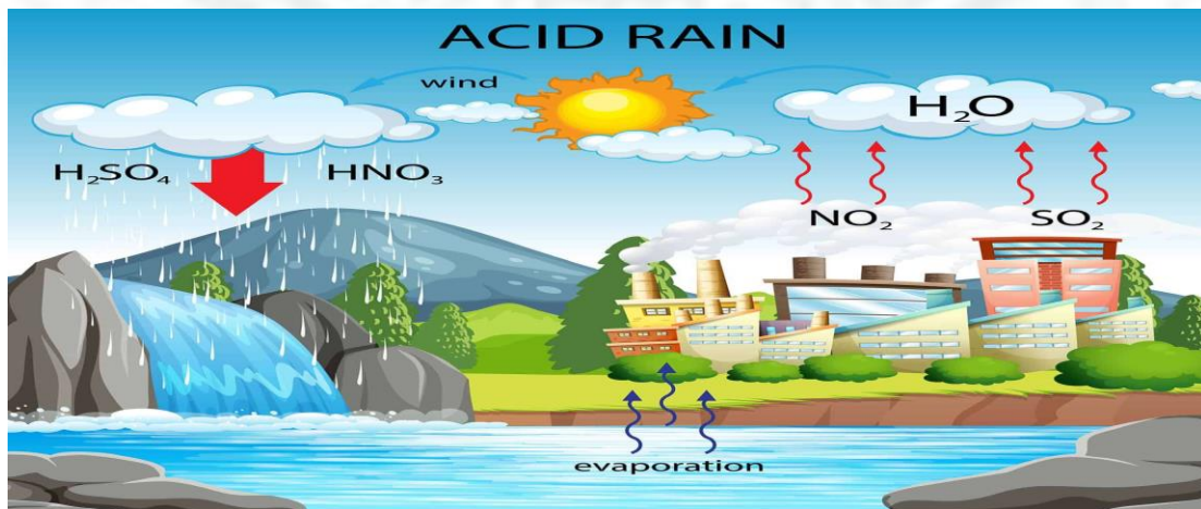
ACID RAIN
