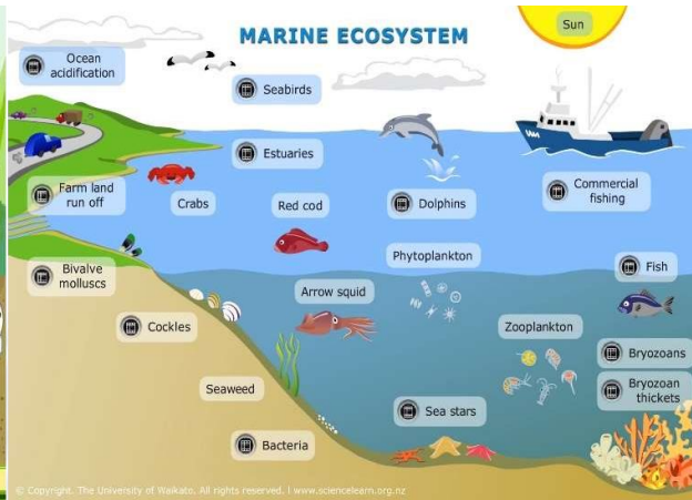
MARINE ECOSYSTEM
