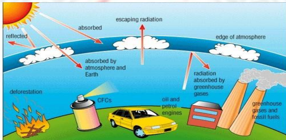
GLOBAL WARMING
