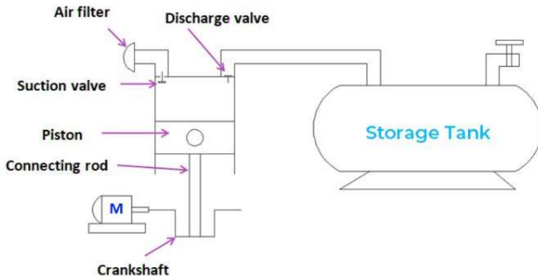
Main Parts of Reciprocating Air Compressor
