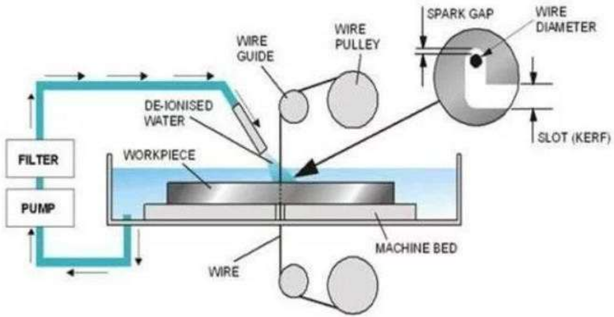
WIRE-CUT EDM PROCESS
