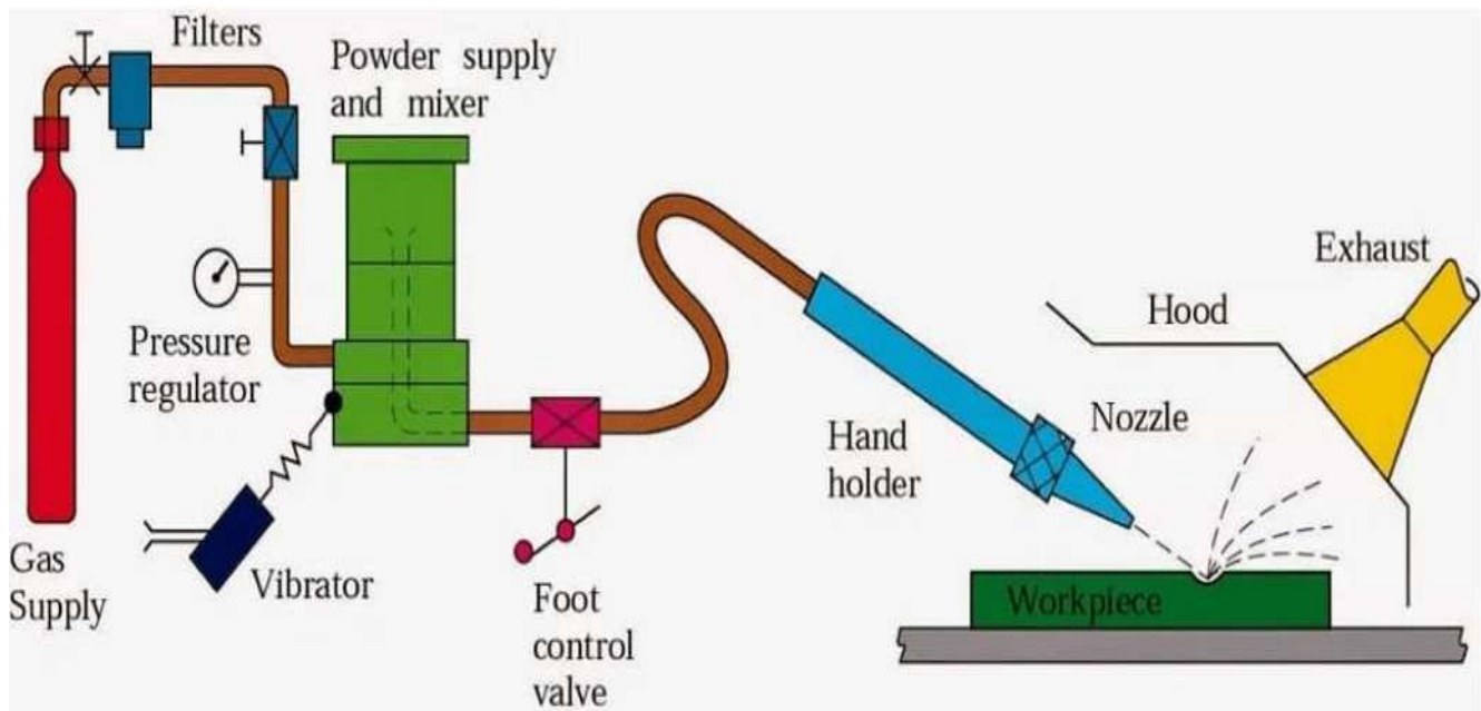
ABRASIVE JET MACHINING PROCESS
