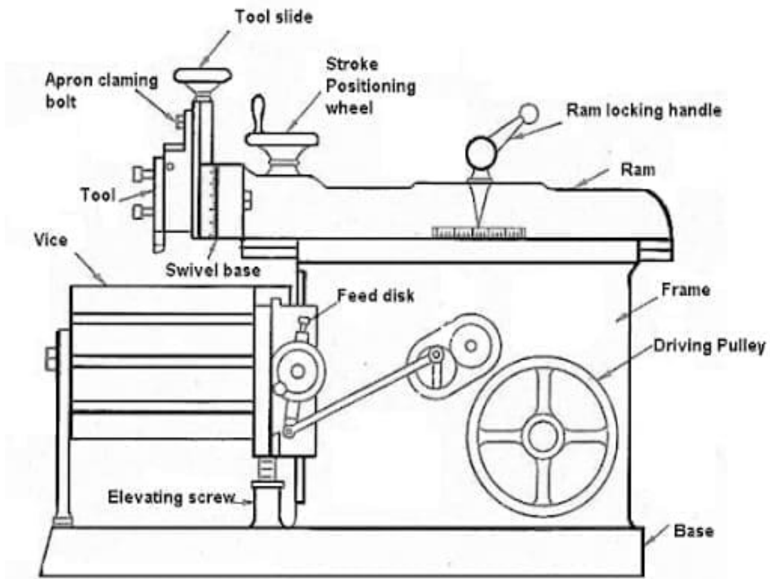
SHAPER MACHINE
