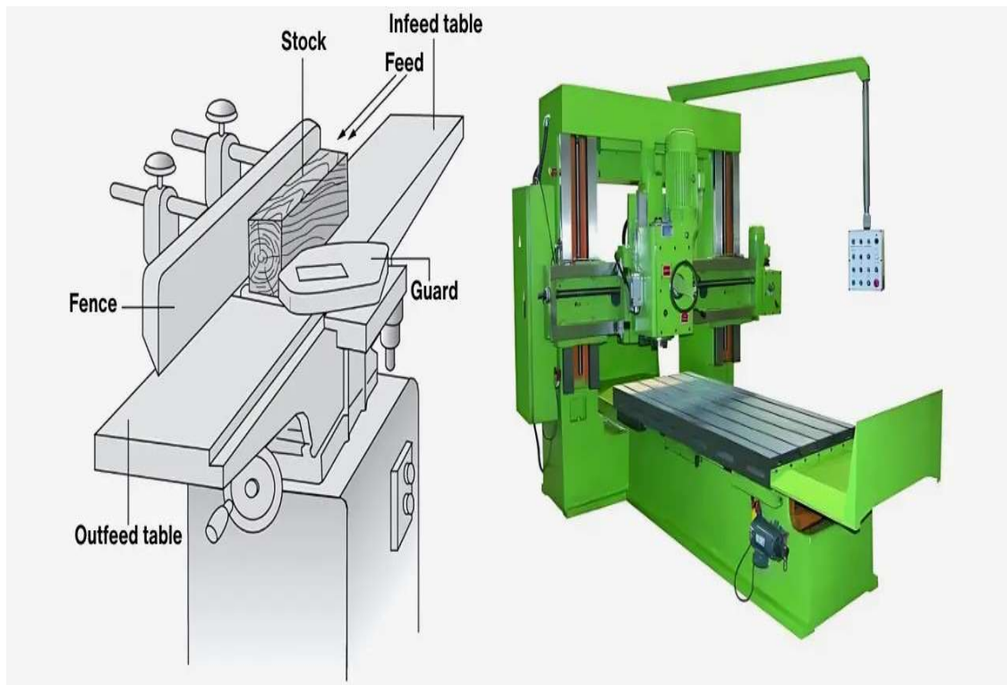
PLANER MACHINE
