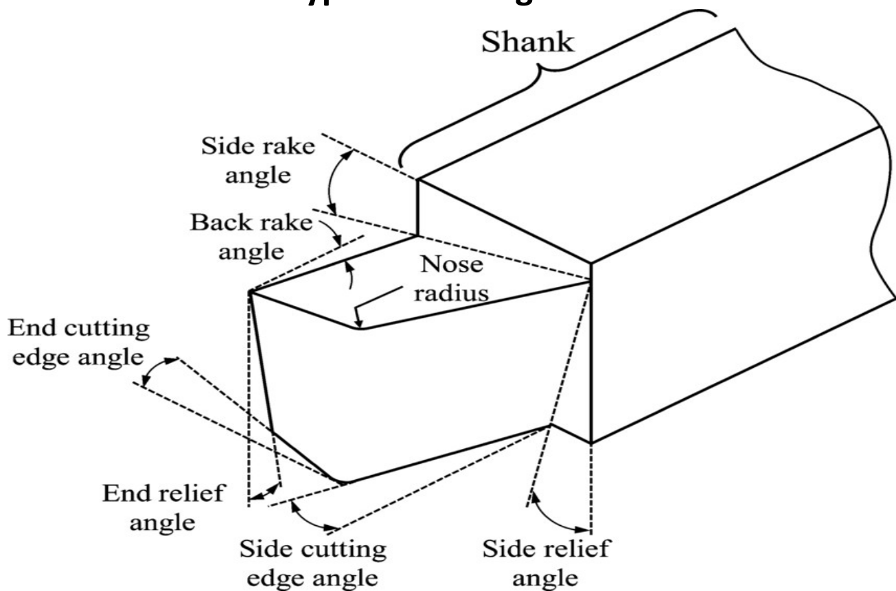
TOOL GEOMETRY
