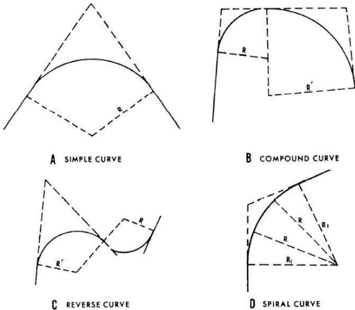
Figure 2.—Horizontal curves.
