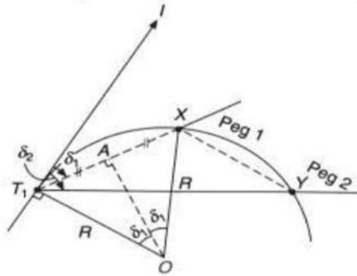
Figure 5 Polar Staking
