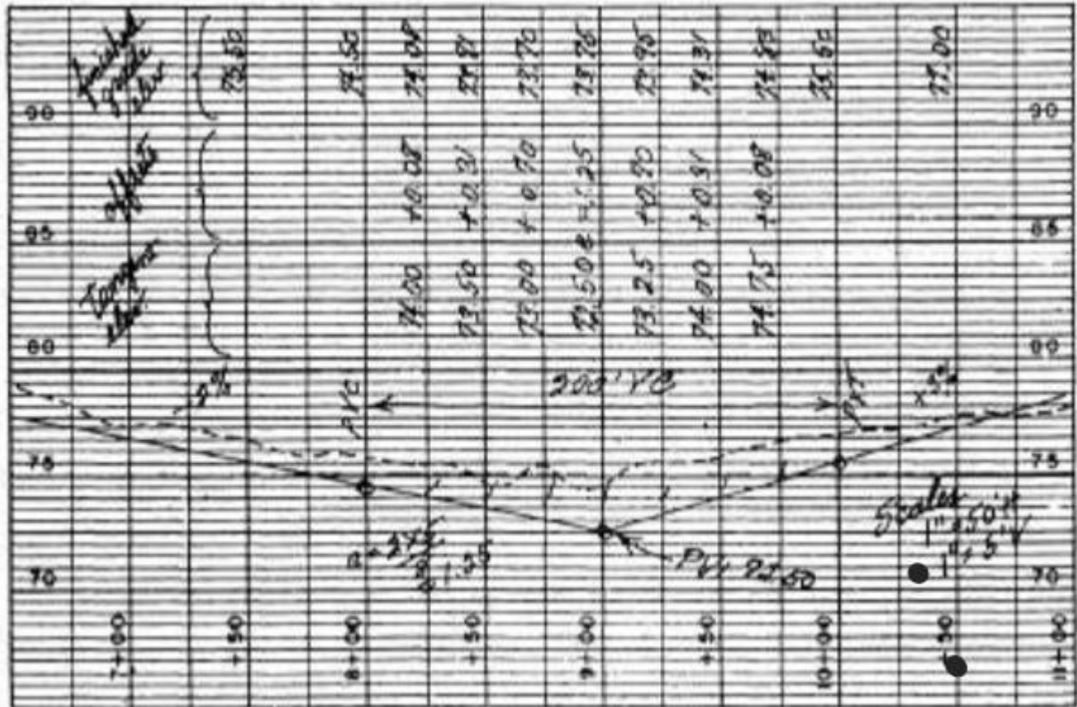
Figure 9 Profile work sheet.
