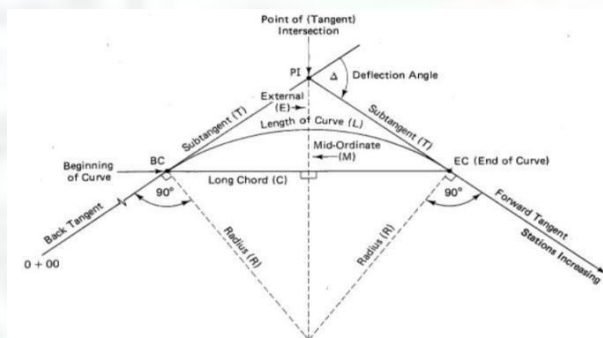
Figure 3 Elements of a Circular Curve
