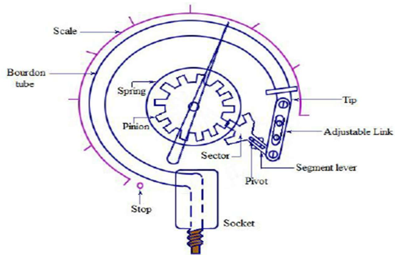
BOURDON TUBE PRESSURE GAUGE
