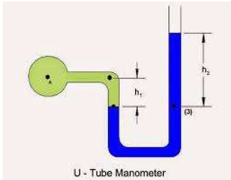
U-TUBE MANOMETER
