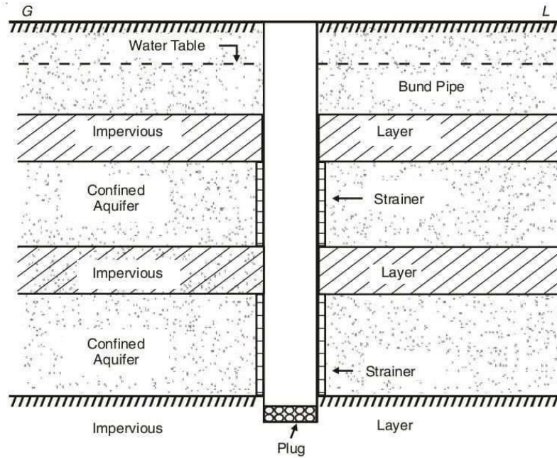
Fig. 8.4. Tube well (Strainer type).
