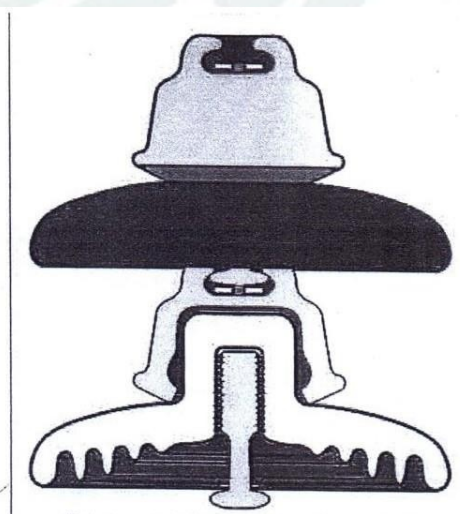
Suspension Disc Insulator
