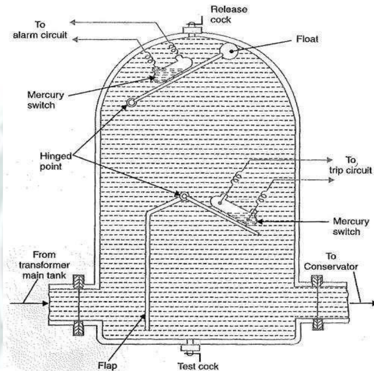
Buchholz relay
